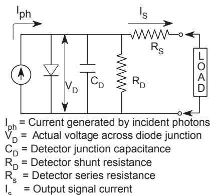
Figure 1 Germanium Photodiode Equivalent Circuit
