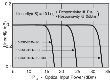
Figure 5 Typical 1550nm High Power Linearity
