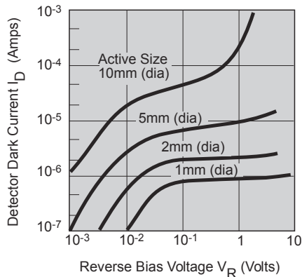
Figure 9 Dark Current vs Reverse Bias Voltage
