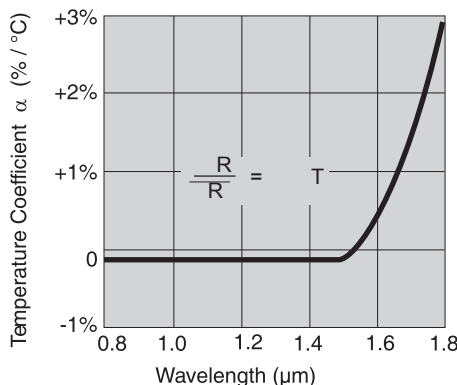
Figure 3 Temperature Coefficient of Responsivity at 25 ^{\circ}\text{C}
