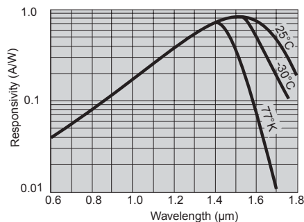
Figure 2 Typical Responsivity for J16 Series Ge
