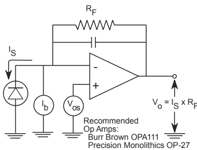
Figure 6 Basic Operating Circuit
