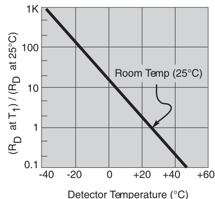
Figure 4 Change in Shunt Resistance vs Temperature
