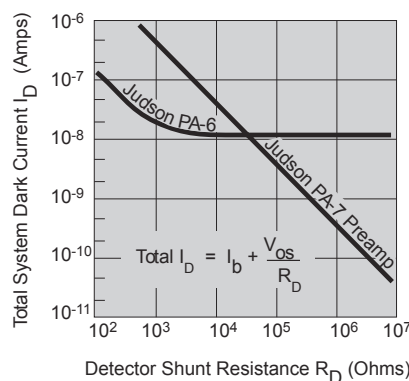
Figure 7 Total Dark Current vs Detector Resistance
