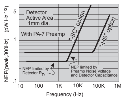
Figure 10 NEP vs Frequency for J16 Device Options
