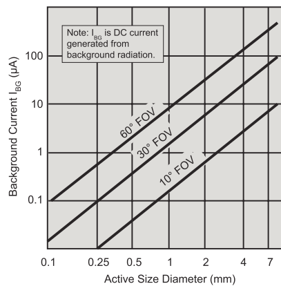
Figure 5 Background Current I_{BG} Current vs Active Size
