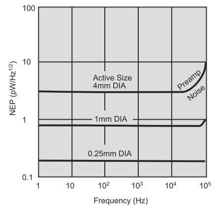
Figure 6 Noise Equivalent Power (NEP) vs Frequency
